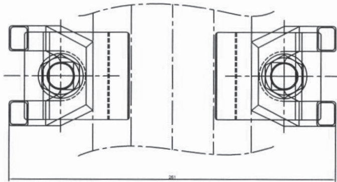
Rail clamp Double Assembly
