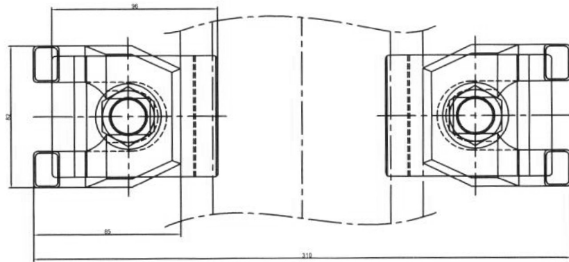
Rail clamp Double Assembly
