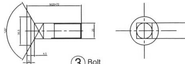
③ Bolt
