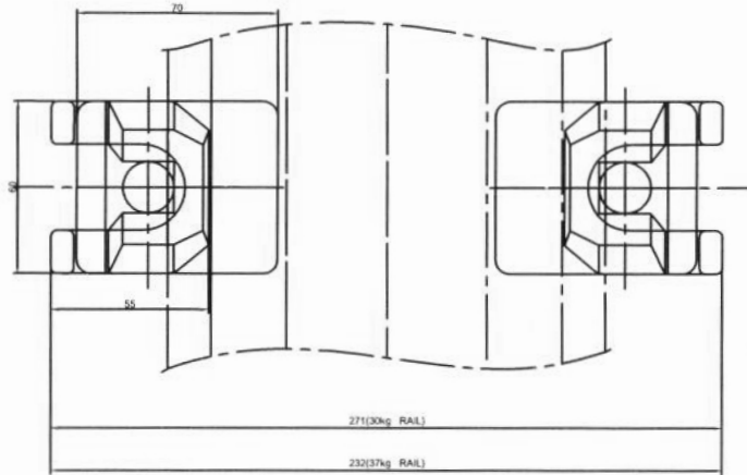
Rail clamp Double Assembly
