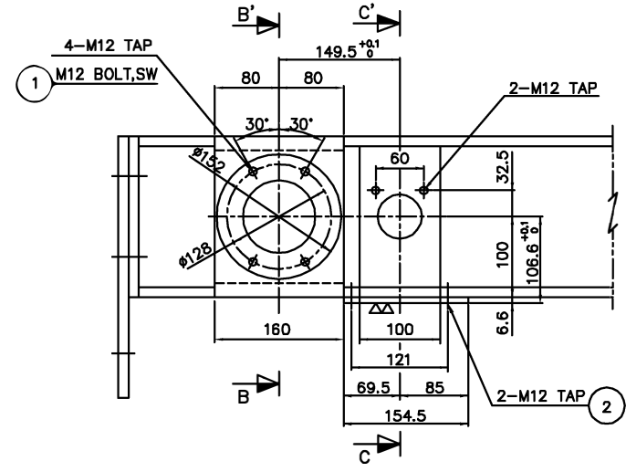
VIEW A-A'
