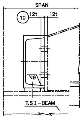
VIEW K-K'
